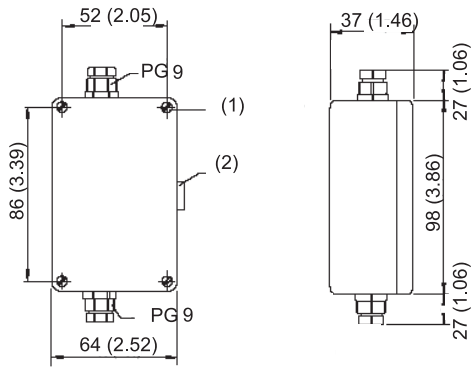
Connection box
